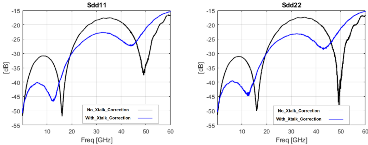
Effect of Xtalk Correction on THRU (ISS 090-0528): I67-GSSG-125um probes
