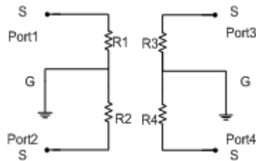
Figure 7. Electrical model
