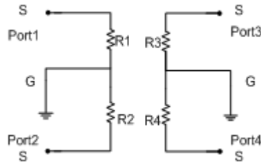
Figure 7. Electrical model
