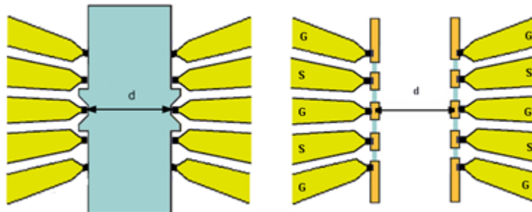
Figure 3. Probe spacing
