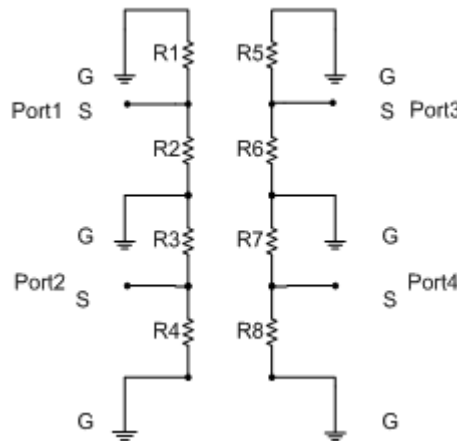
Figure 7. Electrical model
