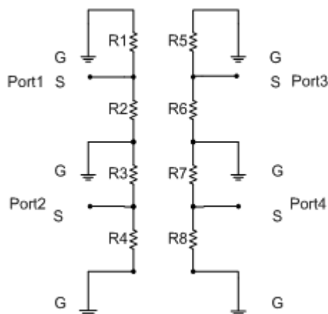
Figure 7. Electrical model
