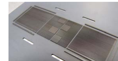
60K+ Apollo fine pitch probe head
