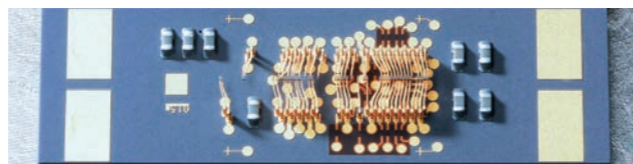
FormFactor's unique "DUTLet" architecture enables superior scrub margin performance, zero soak, wide temperature range, and high speed testing
