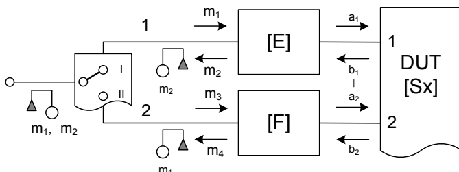
Figure 4. Reference channel VNA.
