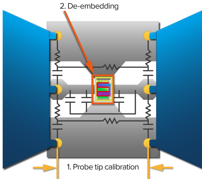
Figure 1. Two-step approach for RF device characterization.
