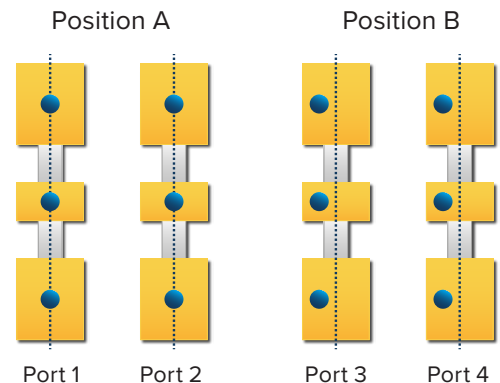
Figure 7. Various positions of the probe tip on the planar Load standard.
